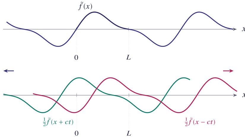
Figure 4.5 The odd periodic extension \tilde{f}(x) and the two waves \frac{1}{2}\tilde{f}(x + ct) and \frac{1}{2}\tilde{f}(x - ct) travelling in opposite directions
