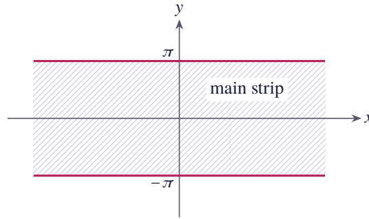
Figure 10.3 The fundamental strip of the hyperbolic functions: -\pi < y \leq \pi
