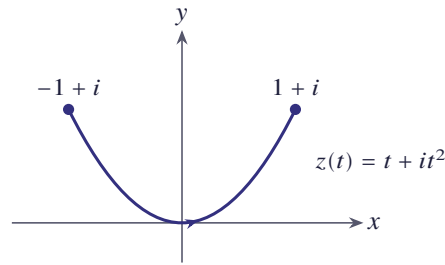
Figure 12.6 The path z(t) = t + it^2 , -1 \leq t \leq 1 , from -1 + i to 1 + i
