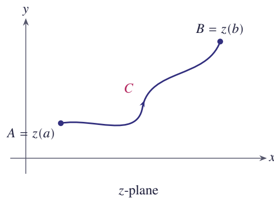
Figure 12.2 The path C , directed from A = z(a) to B = z(b)
