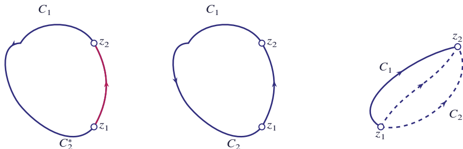
Figure 12.12 The paths C_1 , C_2 and C_2^* ( C_2 with reversed direction) between z_1 and z_2
