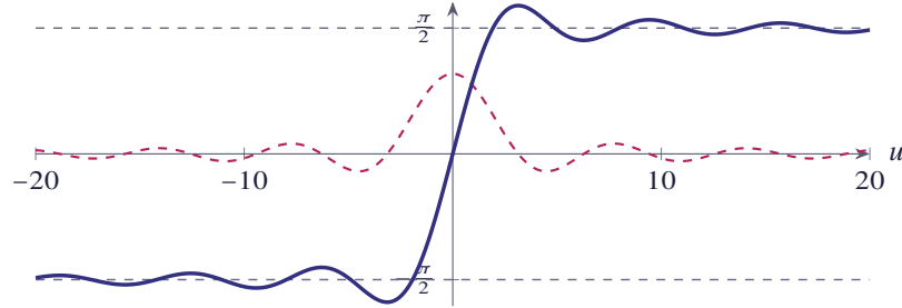
Figure 3.11 The function \text{Si}(u) (solid) and the function \frac{\sin u}{u} (dashed)
