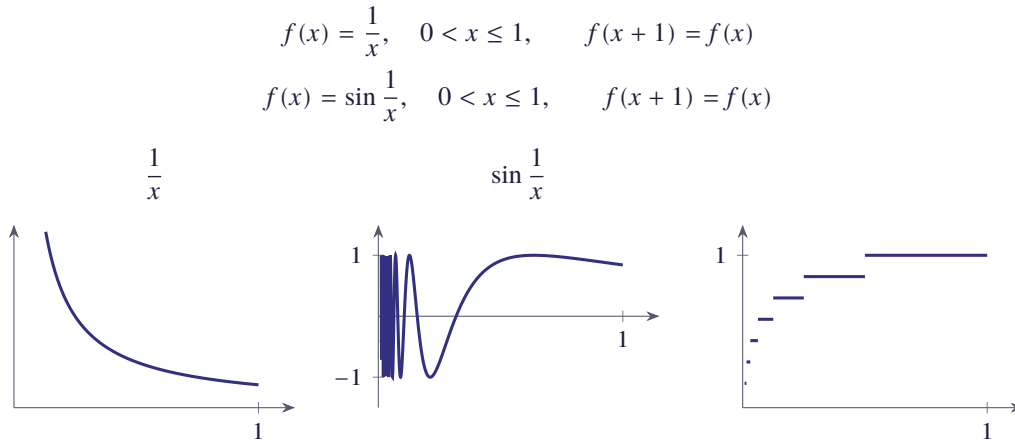
Figure 1.8 Functions that violate Dirichlet's conditions: \frac{1}{x} (unbounded), \sin \frac{1}{x} (infinitely many maxima and minima) and a staircase function with infinitely many steps
