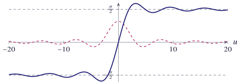
Figure 3.2 The function \text{Si}(u) (solid) and the function \frac{\sin u}{u} (dashed)
