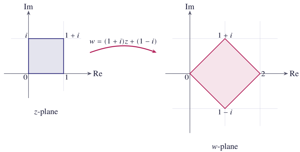
Figure 11.4 The image of the unit square under the mapping w = (1+i)z + (1-i)
