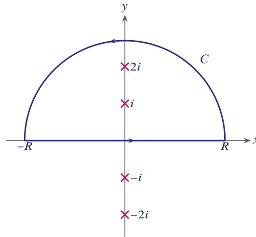
Figure 12.16 The semicircular path; the poles are at z = \pm i and z = \pm 2i
