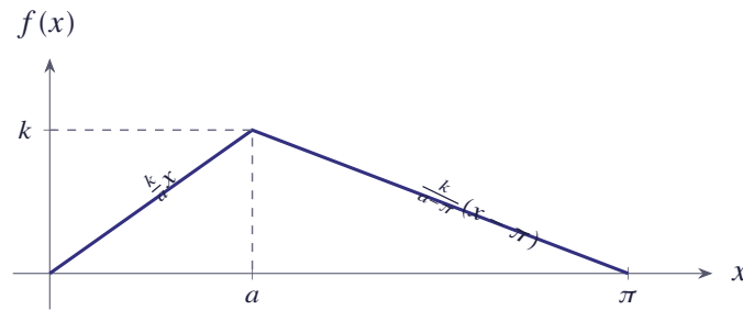
Figure 4.17 The triangular initial profile f(x) with peak value k at x = a
