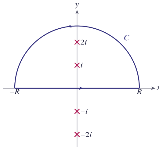
Figure 12.64 The semicircular path; the poles are at z = \pm i and z = \pm 2i
