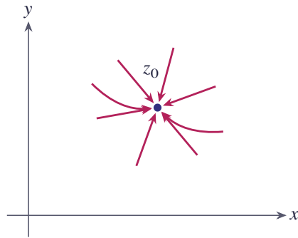
Figure 9.39 Approaching the point z_0 from all directions
