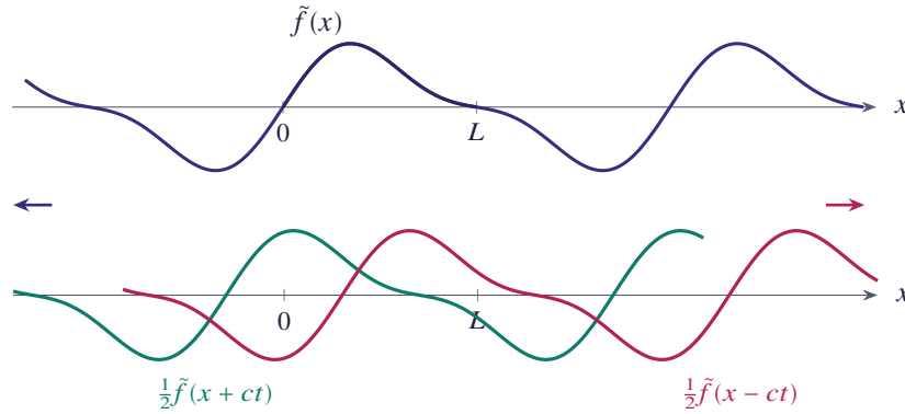
Figure 4.19 The odd periodic extension \tilde{f}(x) and the two waves \frac{1}{2}\tilde{f}(x + ct) and \frac{1}{2}\tilde{f}(x - ct) travelling in opposite directions
