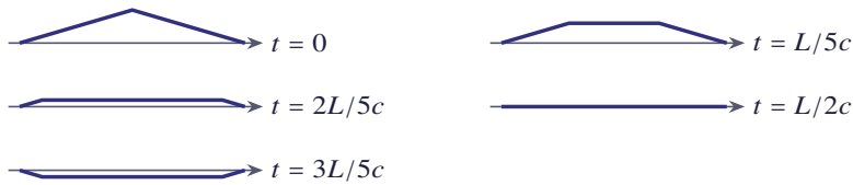
Figure 4.20 The solution of the example at t = 0, L/5c, 2L/5c, L/2c and 3L/5c ; at t = L/2c the string is flat
