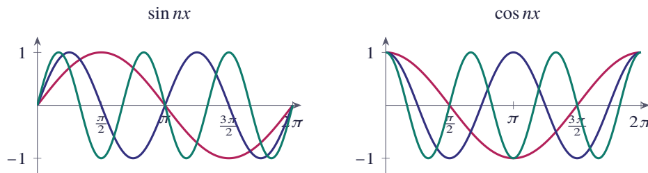
Figure 1.2 The functions \sin nx and \cos nx for n = 1, 2, 3 on [0, 2\pi]
