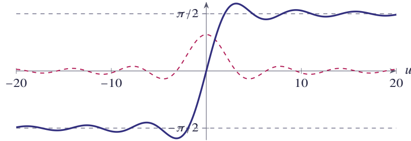
Figure 3.11 The function \text{Si}(u) (solid) and the function \sin u/u (dashed)
