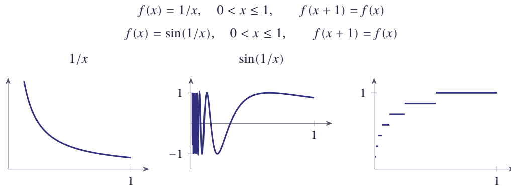
Figure 1.8 Functions that violate Dirichlet's conditions: 1/x (unbounded), \sin(1/x) (infinitely many maxima and minima) and a staircase function with infinitely many steps
