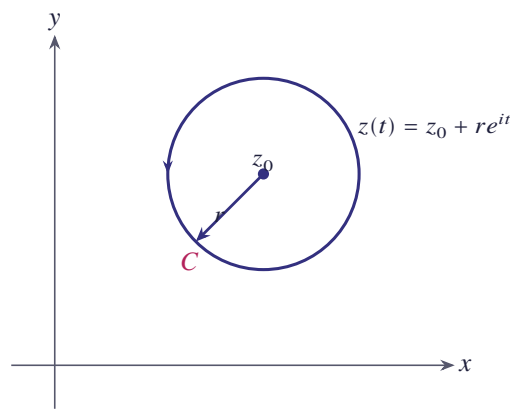
Figure 12.61 A circle C with centre z_0 and radius r
