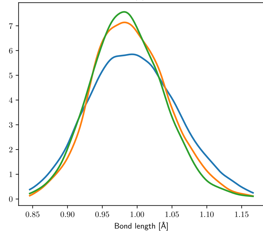
KDE: O – H(1) Bond Length
