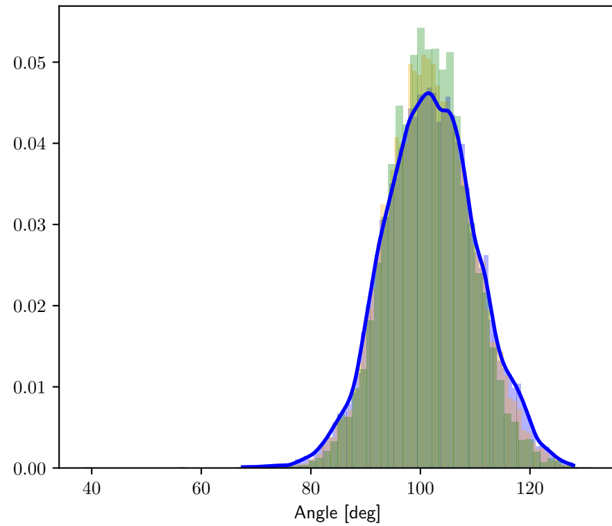
H – O – H Angle Distribution
