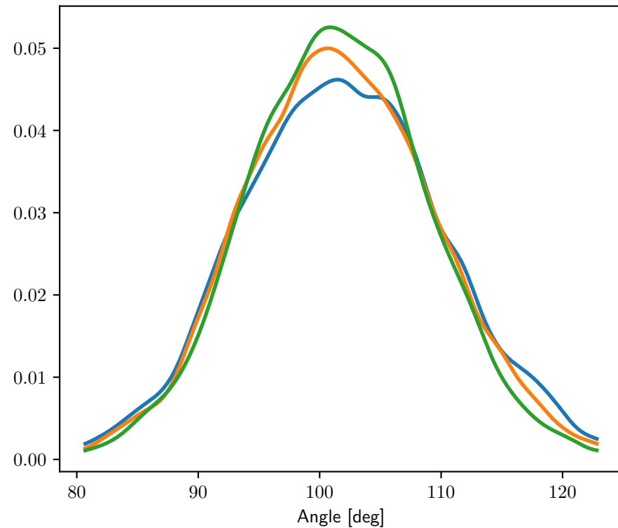
KDE: H – O – H Angle
