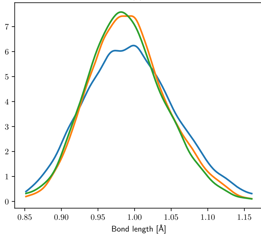
KDE: O – H(2) Bond Length
