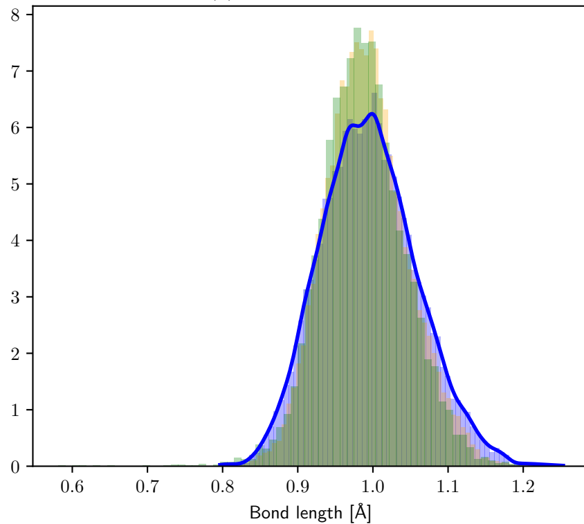
O – H(2) Bond Length Distribution
