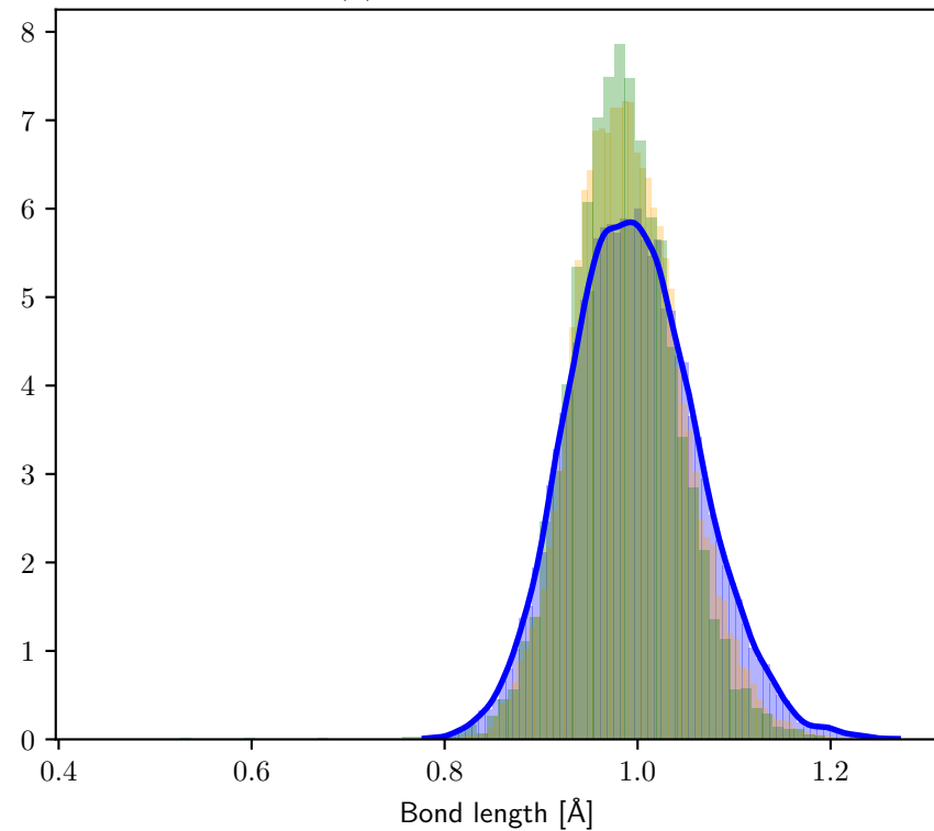
O – H(1) Bond Length Distribution
