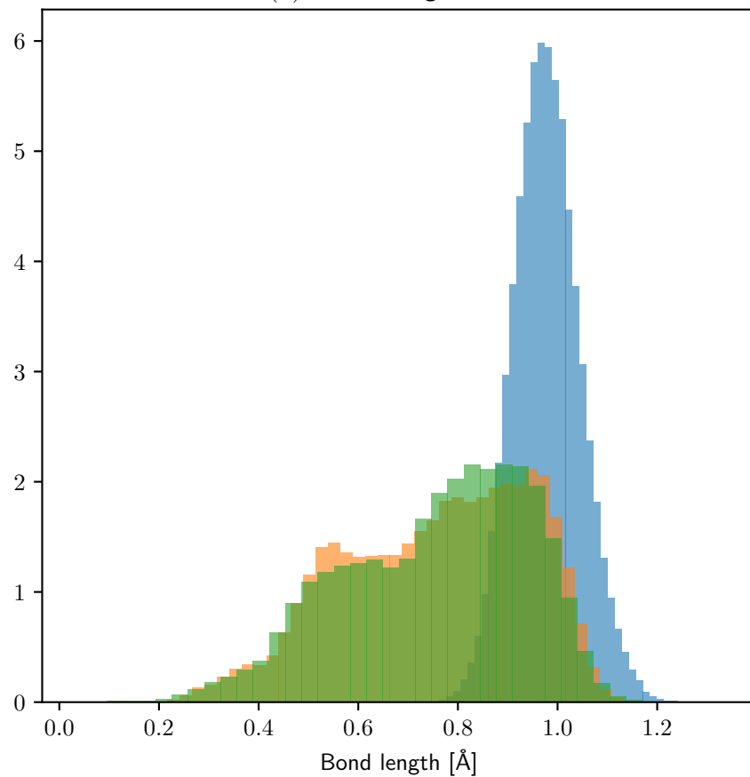
O – H(2) Bond Length Distribution
