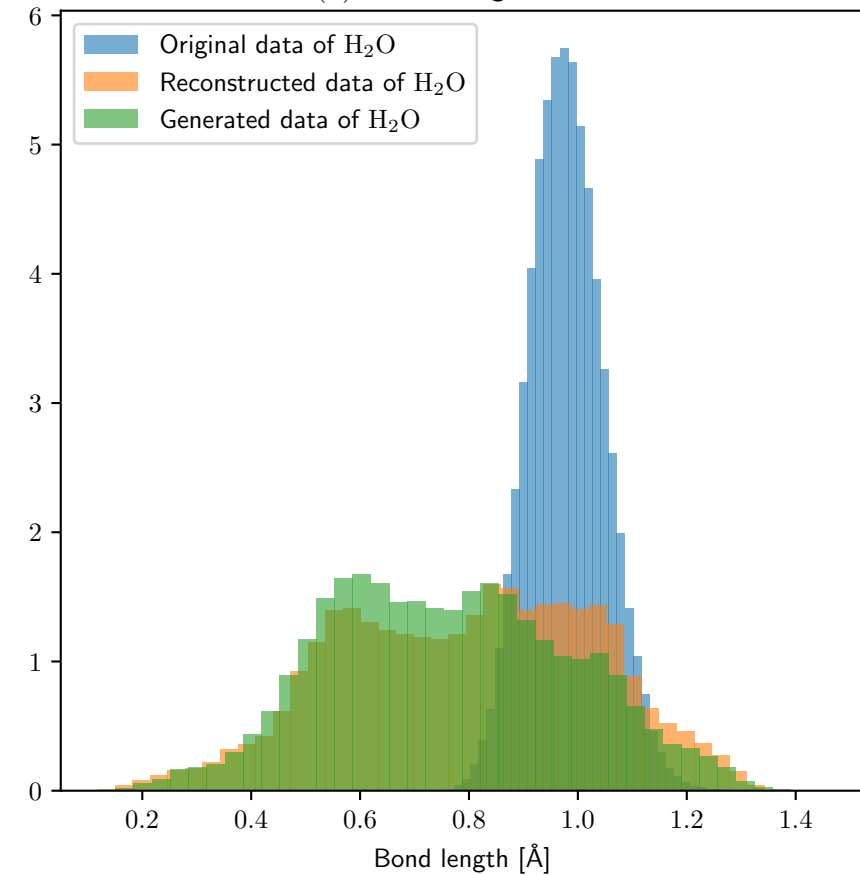
O – H(1) Bond Length Distribution
