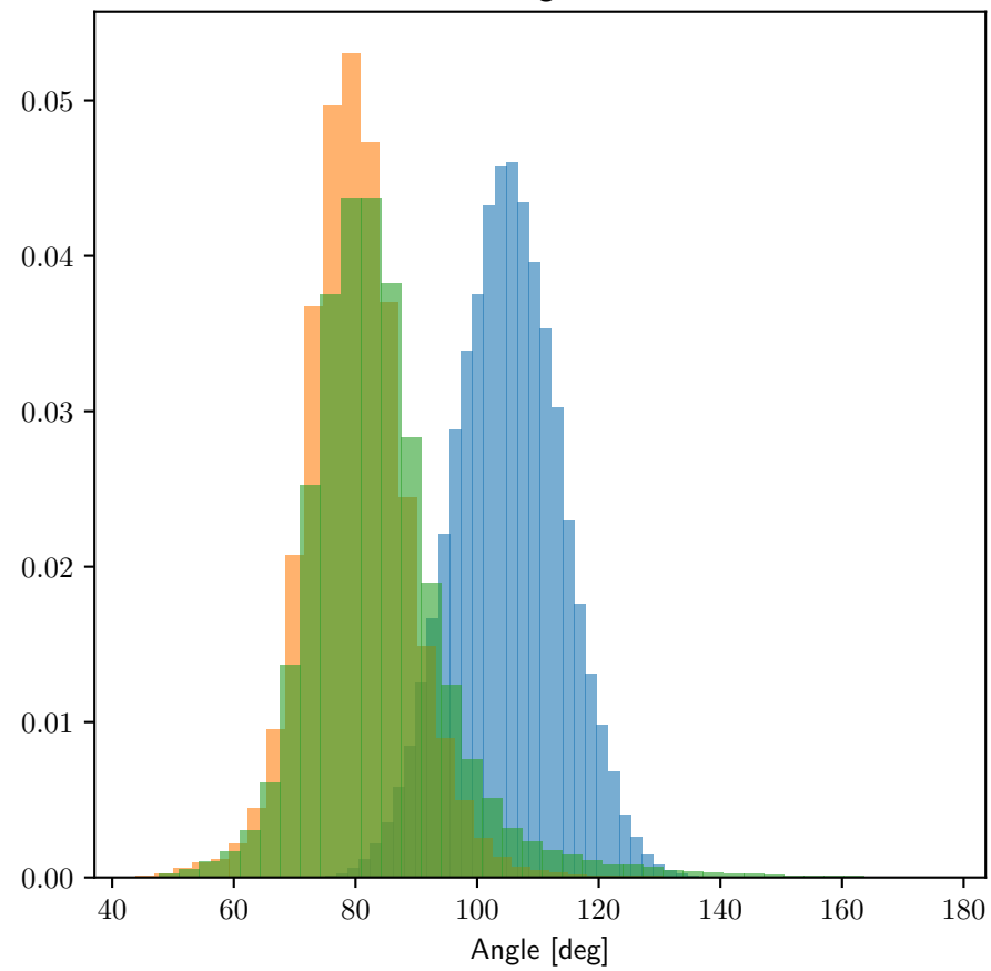
H – O – H Angle Distribution
