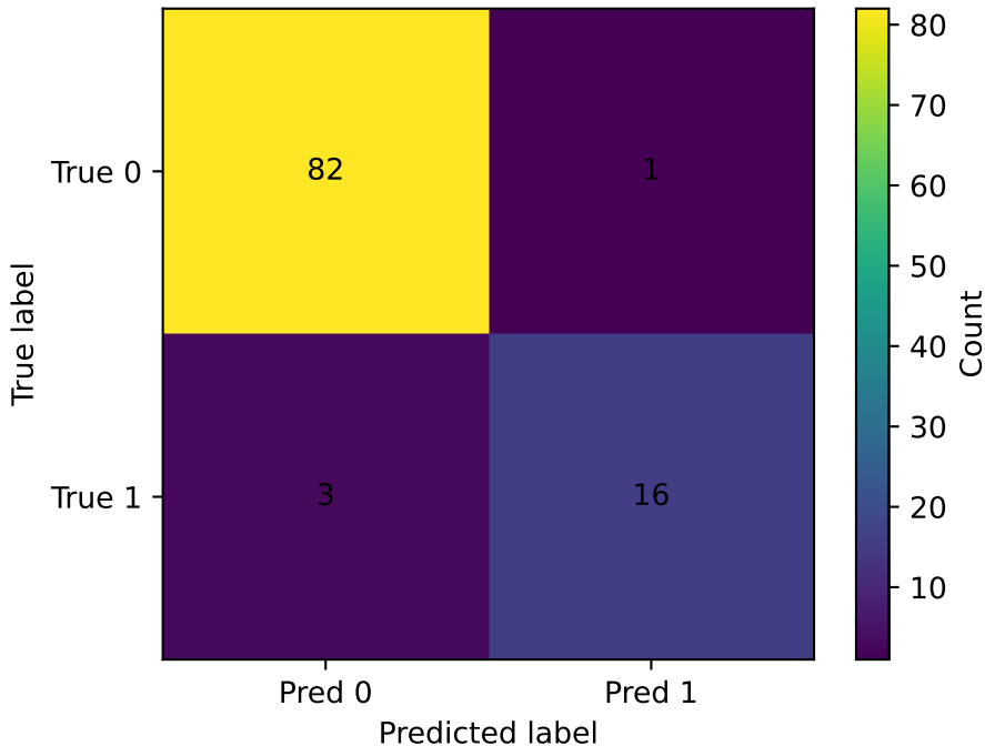
Confusion Matrix, threshold=0.4
