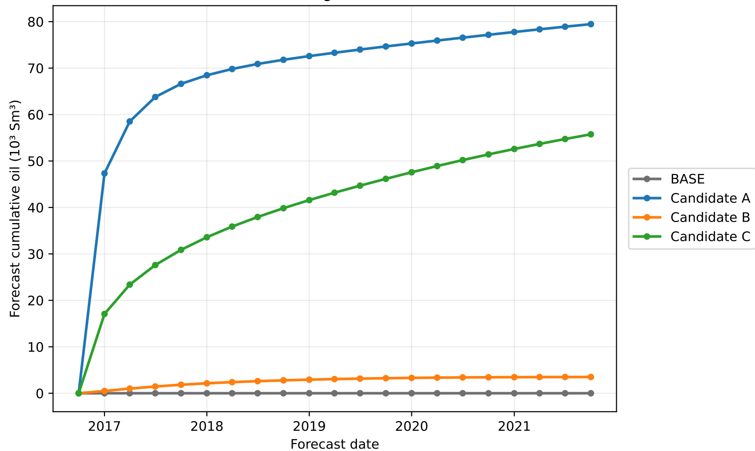
Standalone Infill Screening — Five-Year Cumulative Oil
