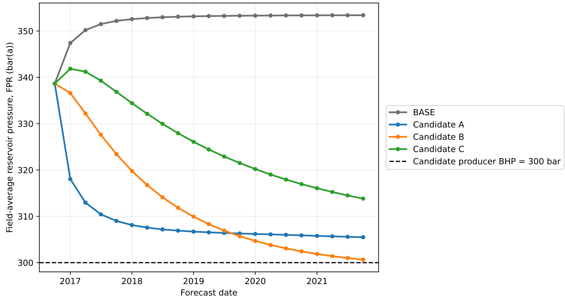
Standalone Infill Screening — Field-Average Pressure Response
