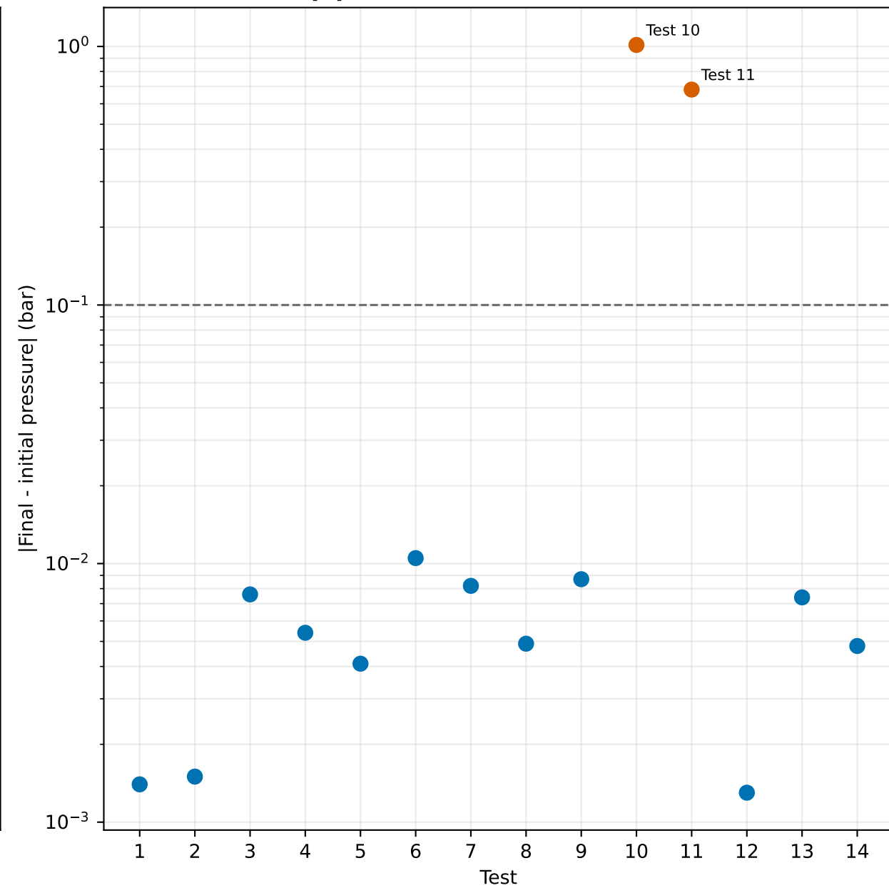
B. End-of-buildup pressure closure
