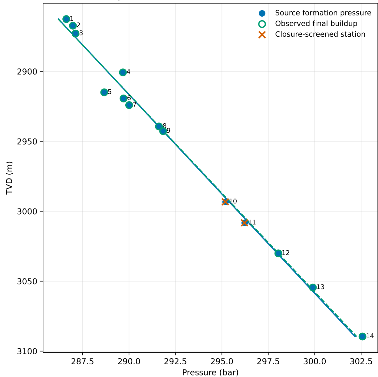
A. Formation pressure versus TVD
