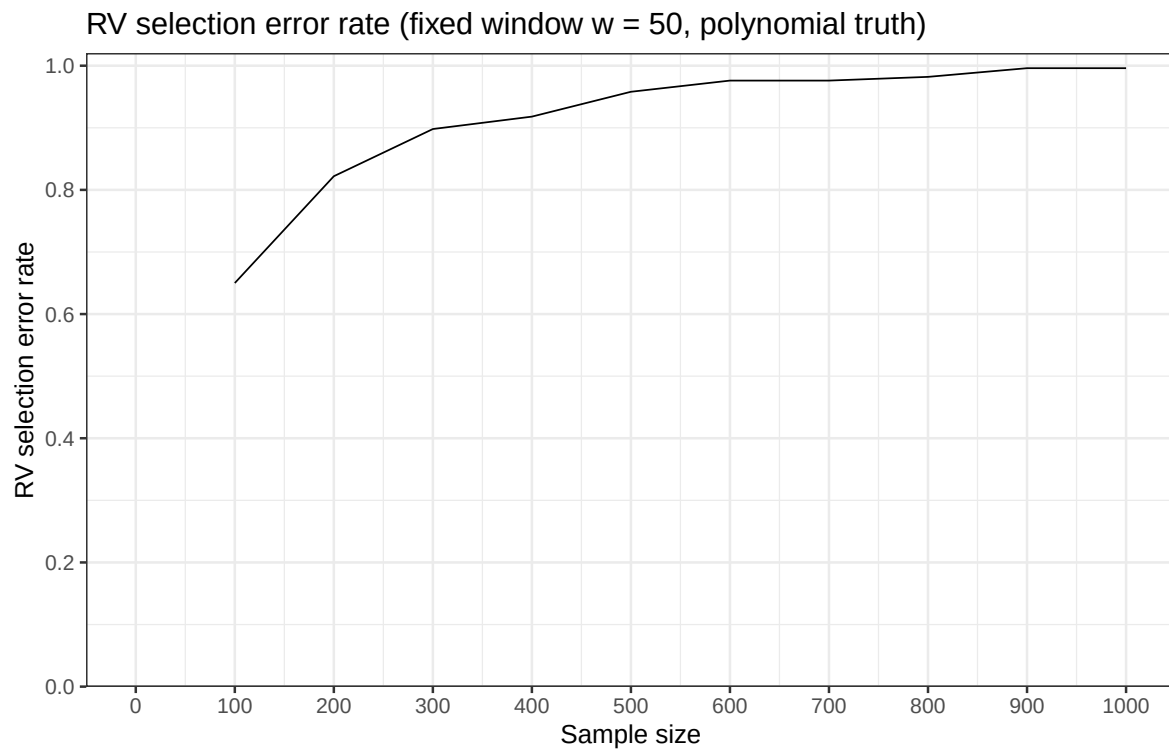
Figure 2: RV selection error rate under polynomial truth (fixed window w = 50 ).
