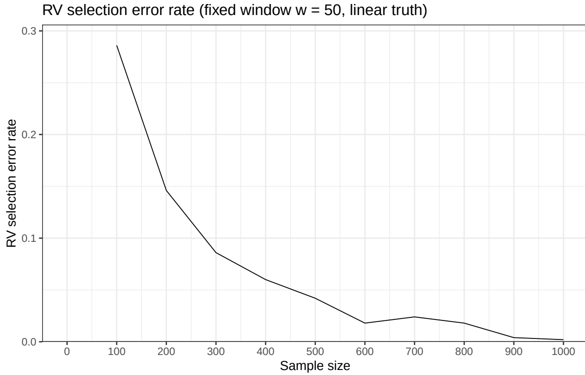
Figure 1: RV selection error rate under linear truth (fixed window w = 50 ).
