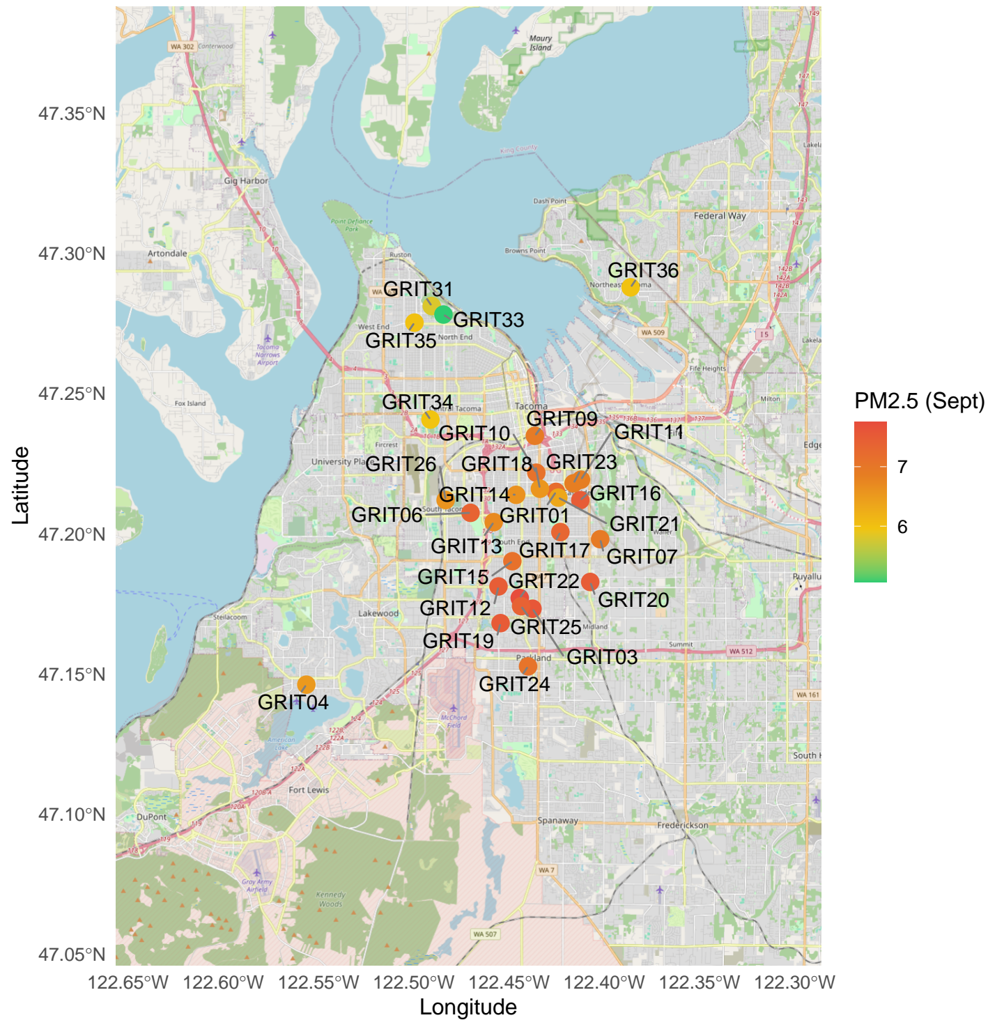
Tacoma points colored by PM2.5 (September)
