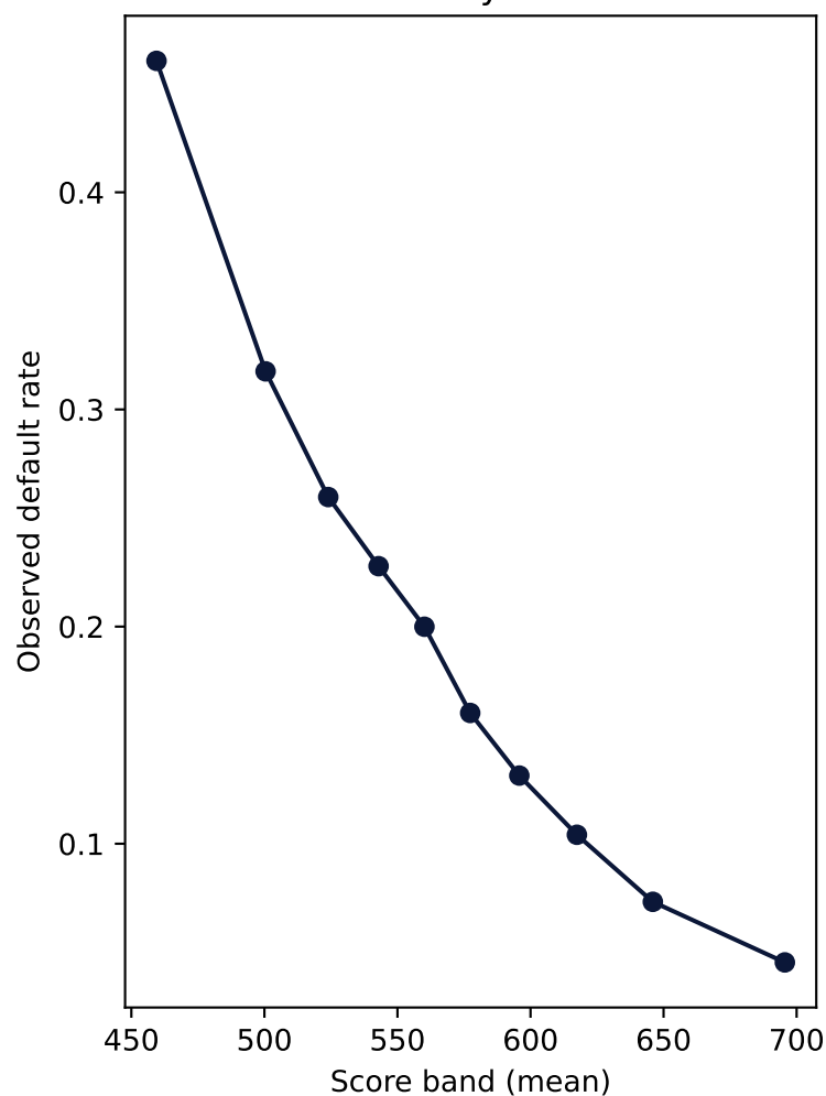
Default rate by score band
