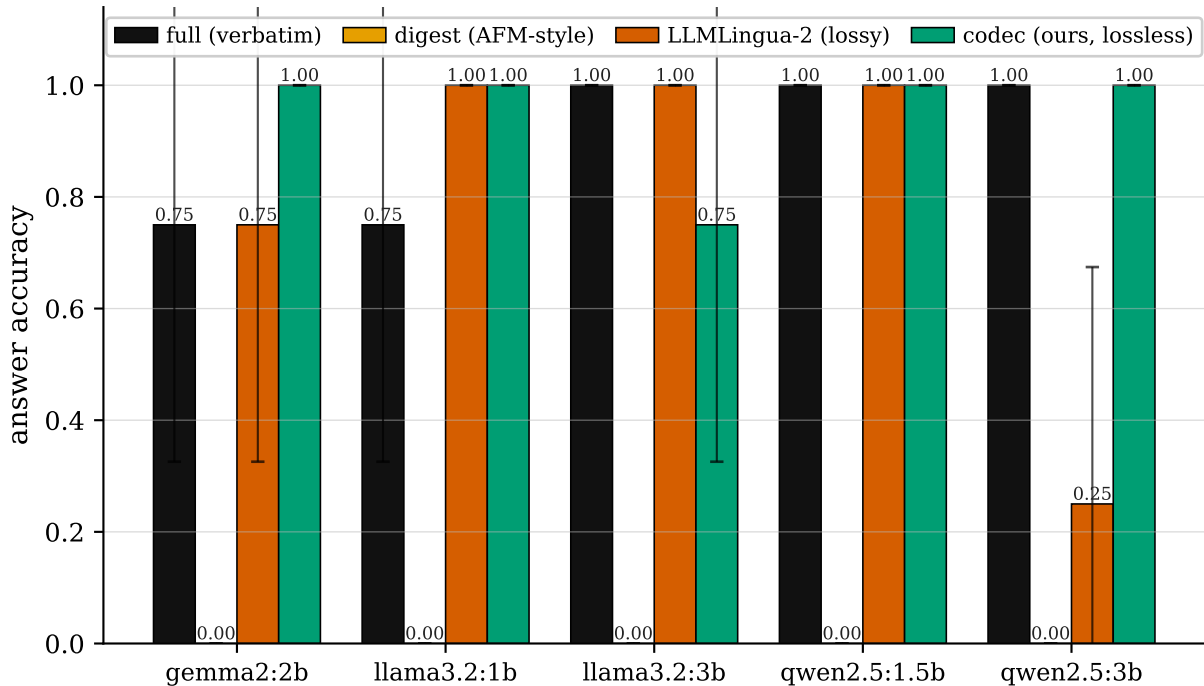
Per-model accuracy: the codec is consistent; LLMingua-2 swings 0.25--1.00
