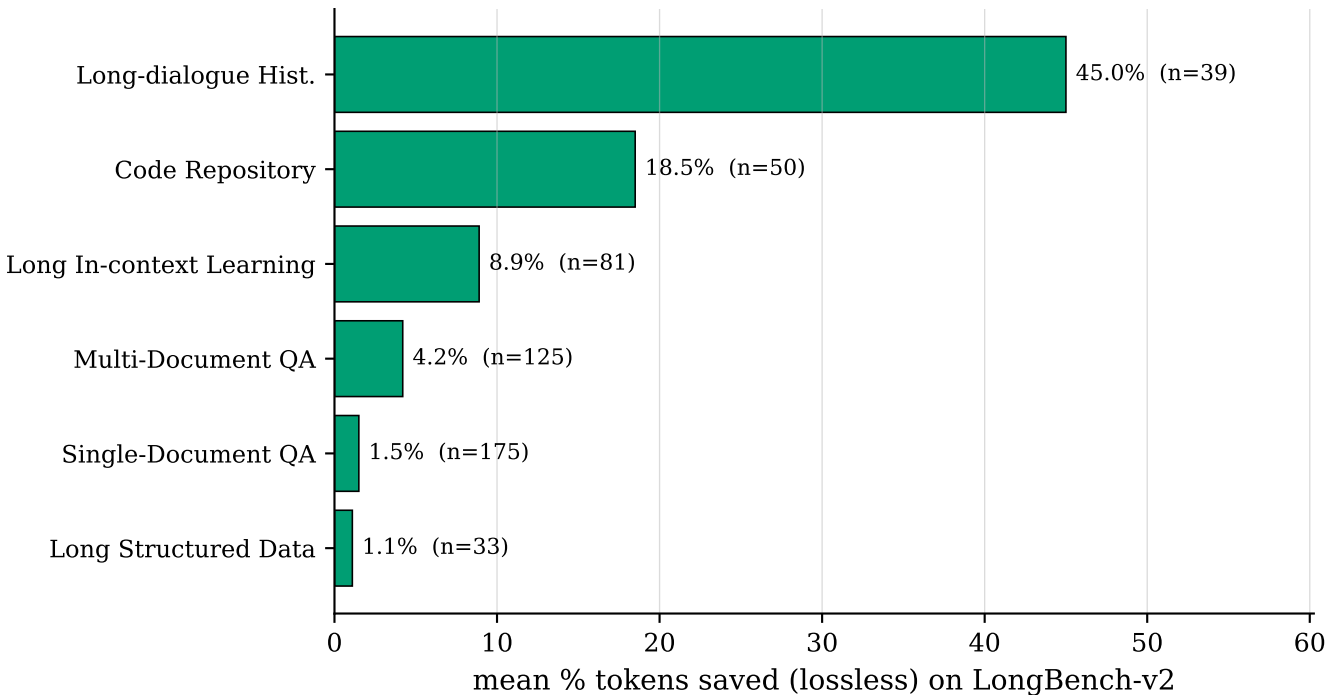
LongBench-v2: codec saving tracks each domain's real redundancy (all lossless)
