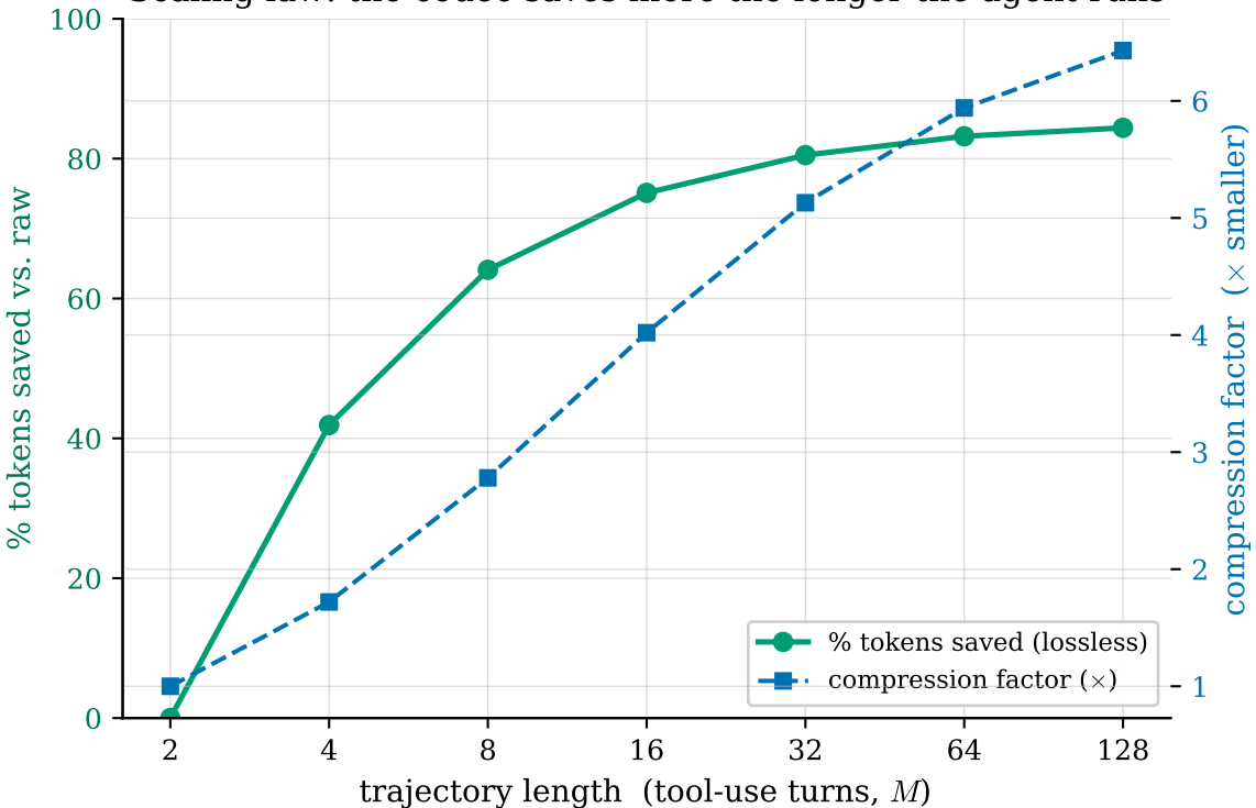
Scaling law: the codec saves more the longer the agent runs
