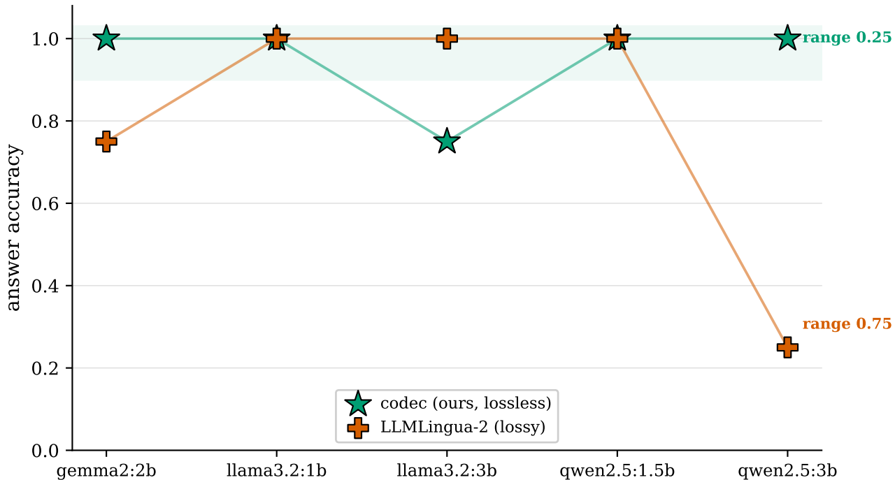
Reliability across models: the codec is tight and high; LLMLingua-2 is not
