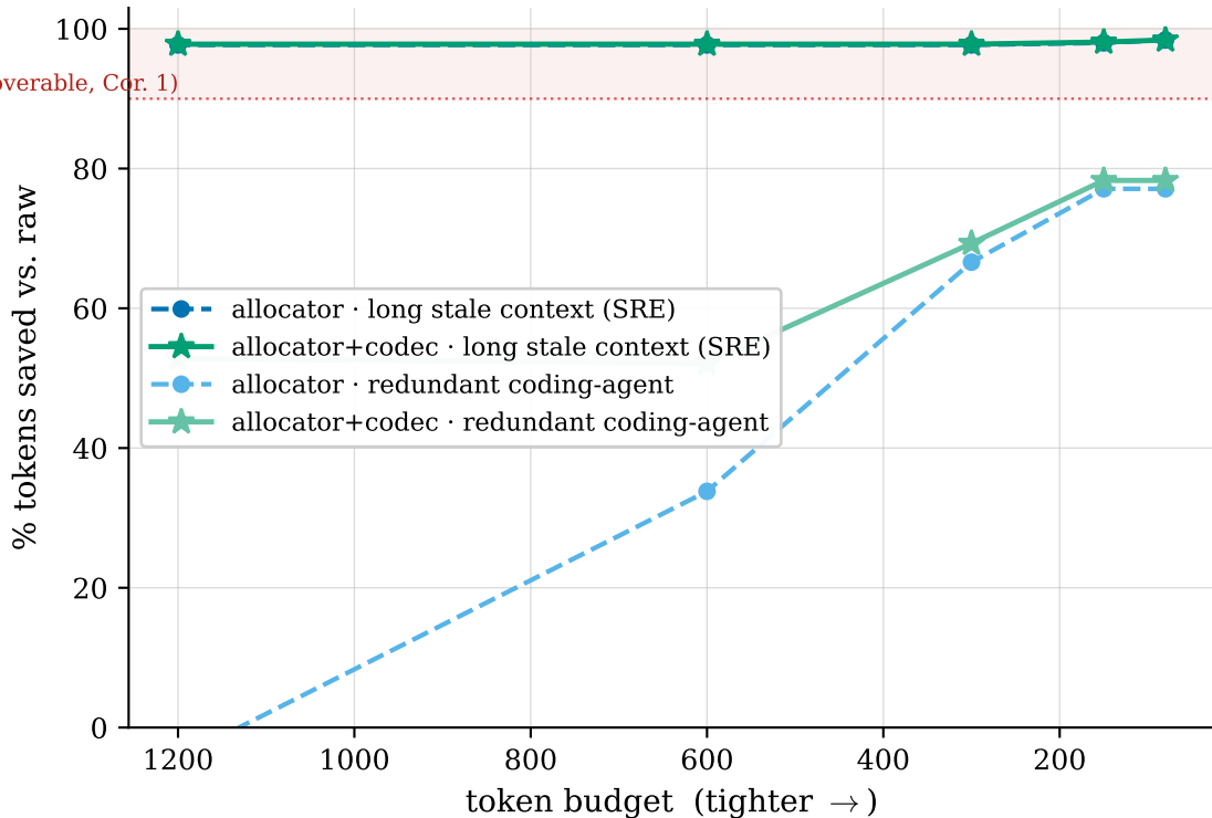
Composed stack: compression ratio climbs as the budget tightens
