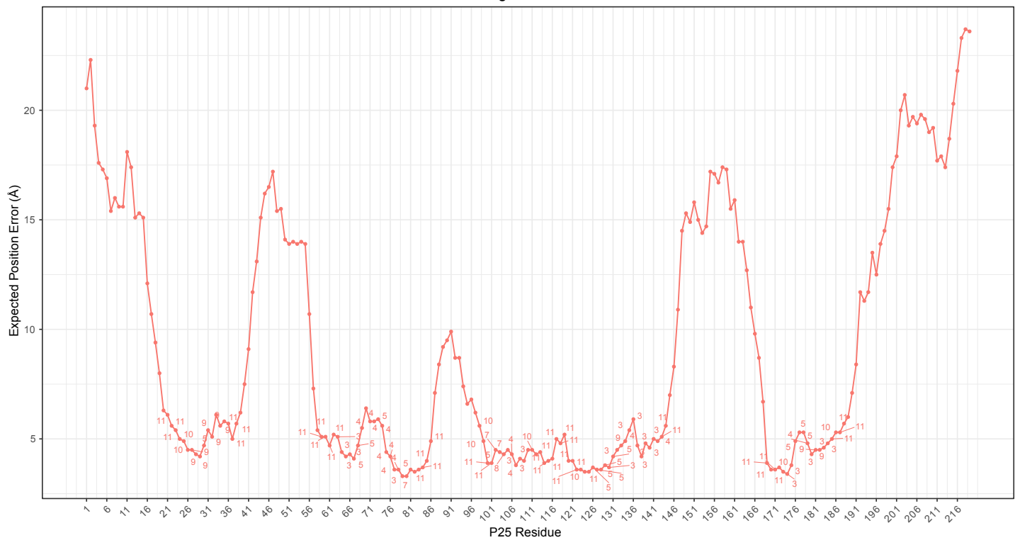
P25 binding to 28nt ssDNA
