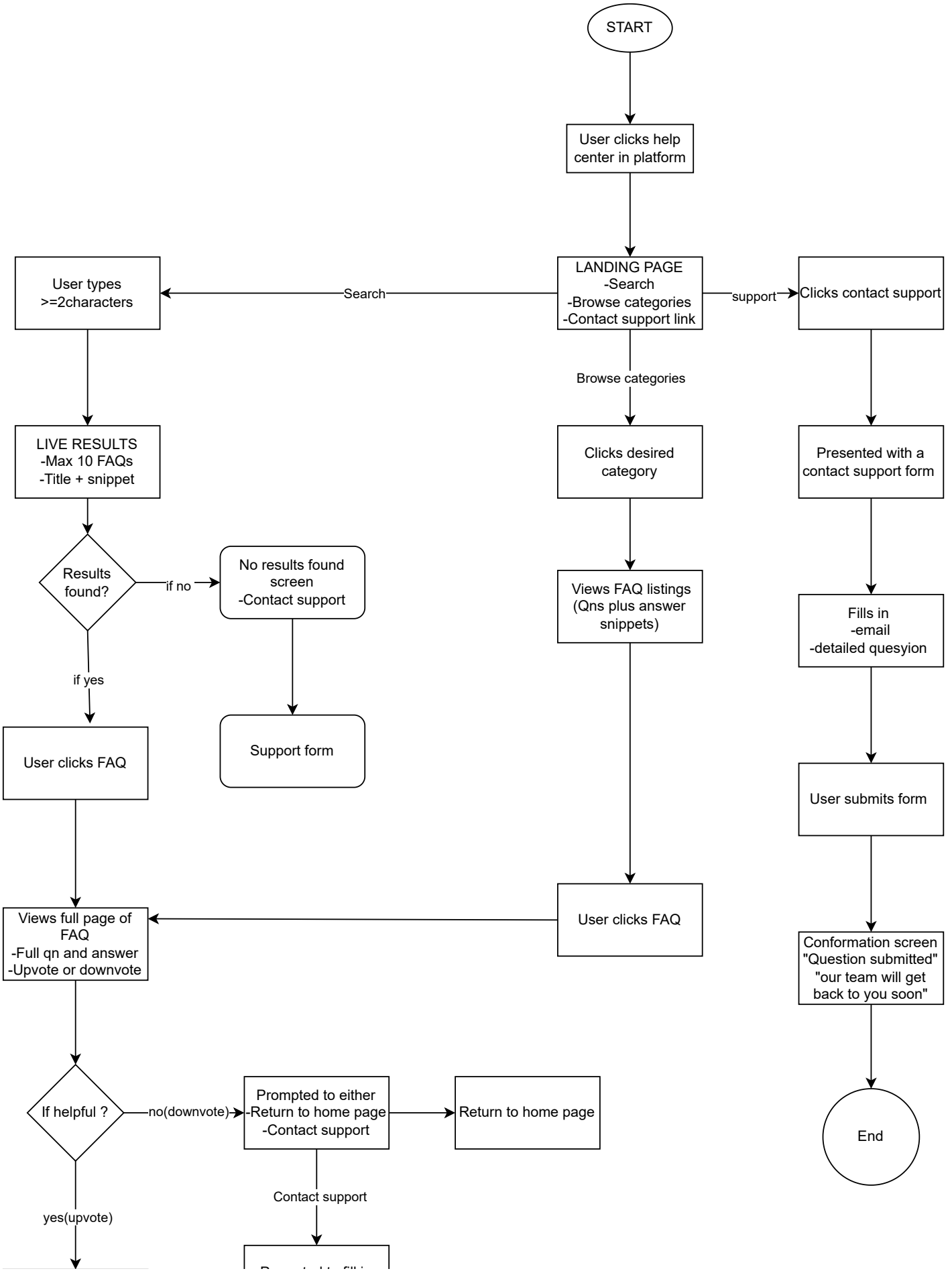
User flow diagram
