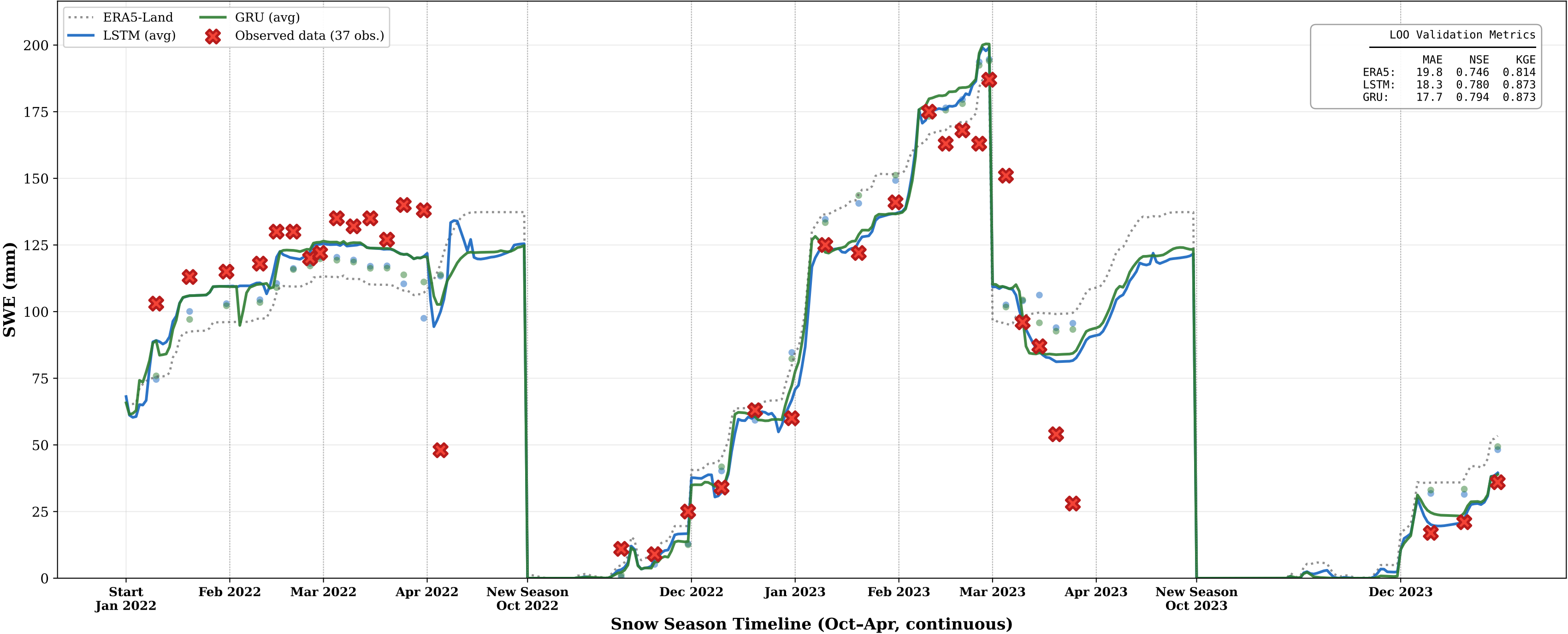
LSTM / GRU Bias-Corrected SWE Predictions LSTM: MAE=18.3 mm, NSE=0.780 | GRU: MAE=17.7 mm, NSE=0.794 | ERA5: MAE=19.8 mm
