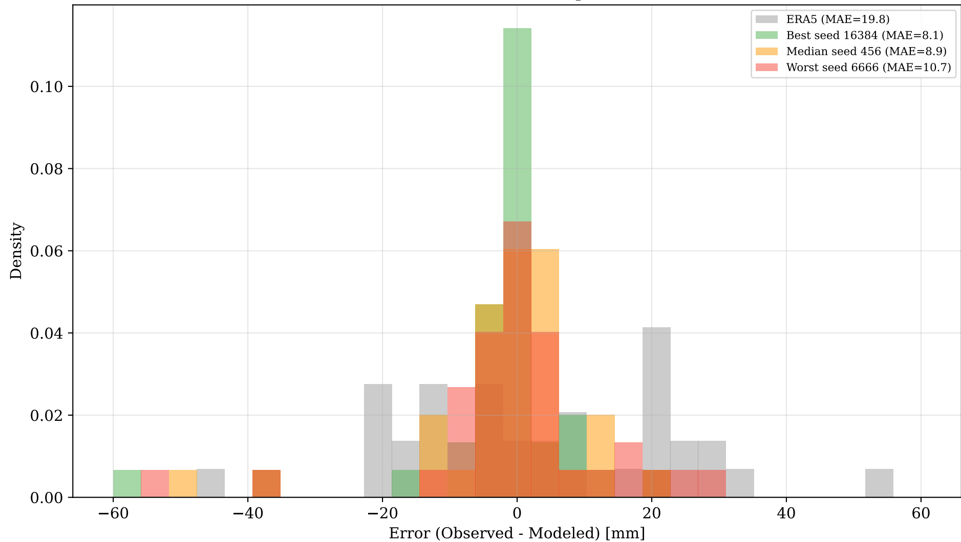
Error Distributions: ERA5 vs Representative Seeds
