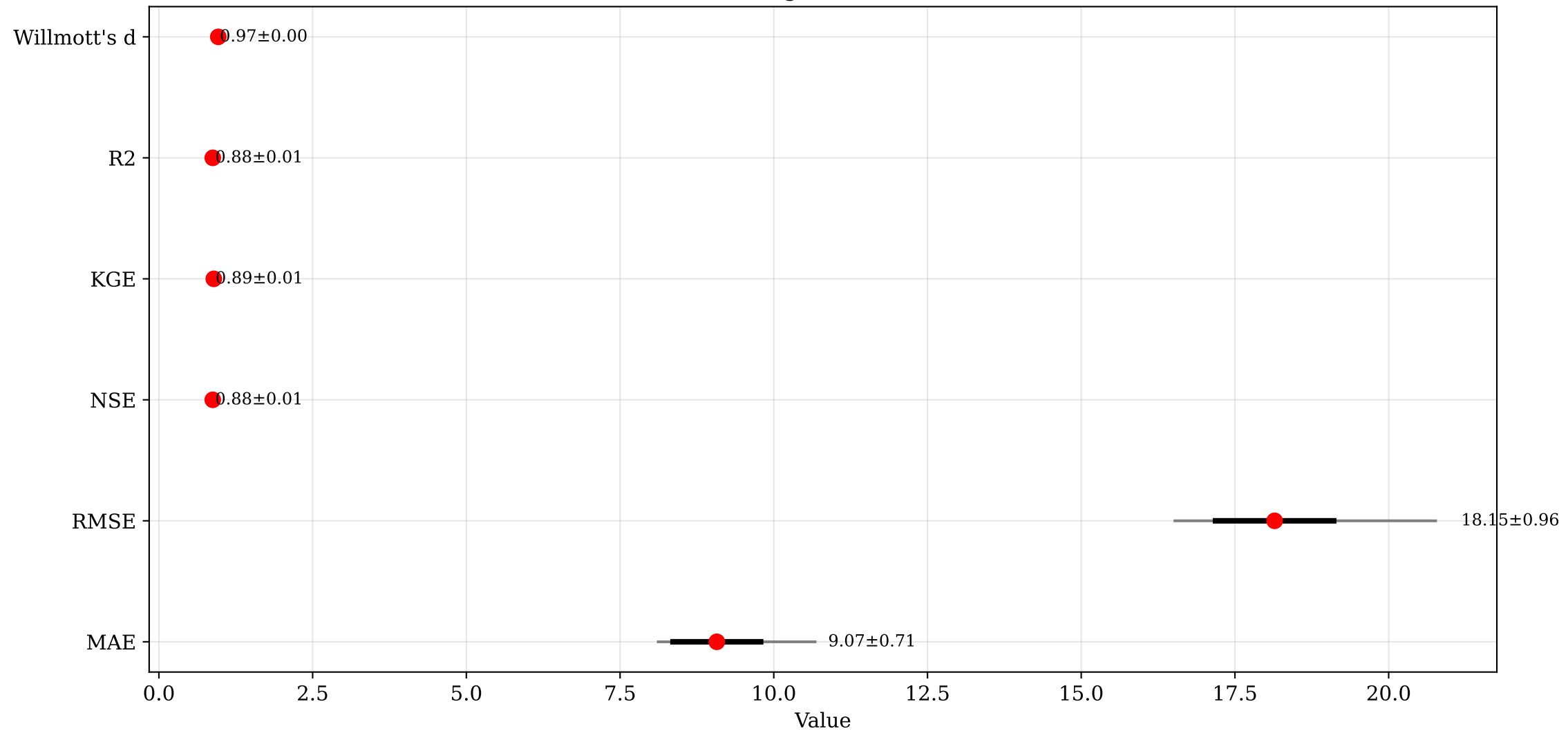
Mean \pm Std and Range of Metrics Across Seeds
