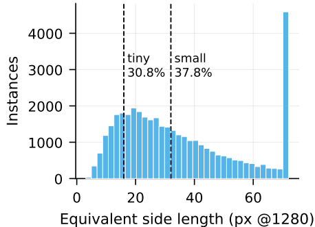
(b) Scale: 68.6% below 32px
