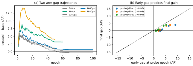
Fig. 2. Online two-arm prediction test. (a) Best-checkpoint gap trajectories (rebalanced — base) per resolution; (b) early probe gap versus final gain—a 30-epoch probe attains r=0.98 and a 2.5-AP threshold separates larger-gap regimes from the volume-saturated 1280-px regime in 5/5 cases.
