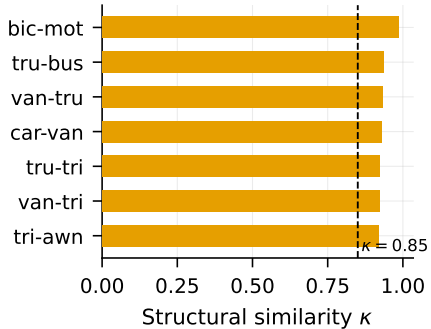
(c) Structurally confusable pairs
