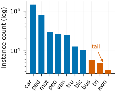
(a) Long-tail: 44.6:1 head-tail ratio
