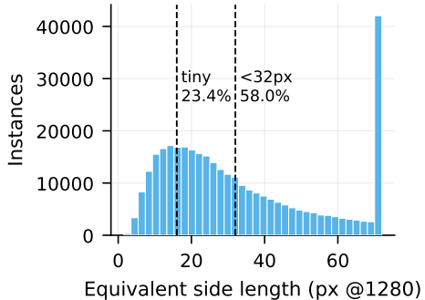
(b) Scale: 58.0% below 32px (1280-ratio)
