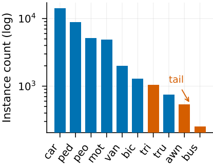
(a) Long-tail: 45:1 head-tail ratio
