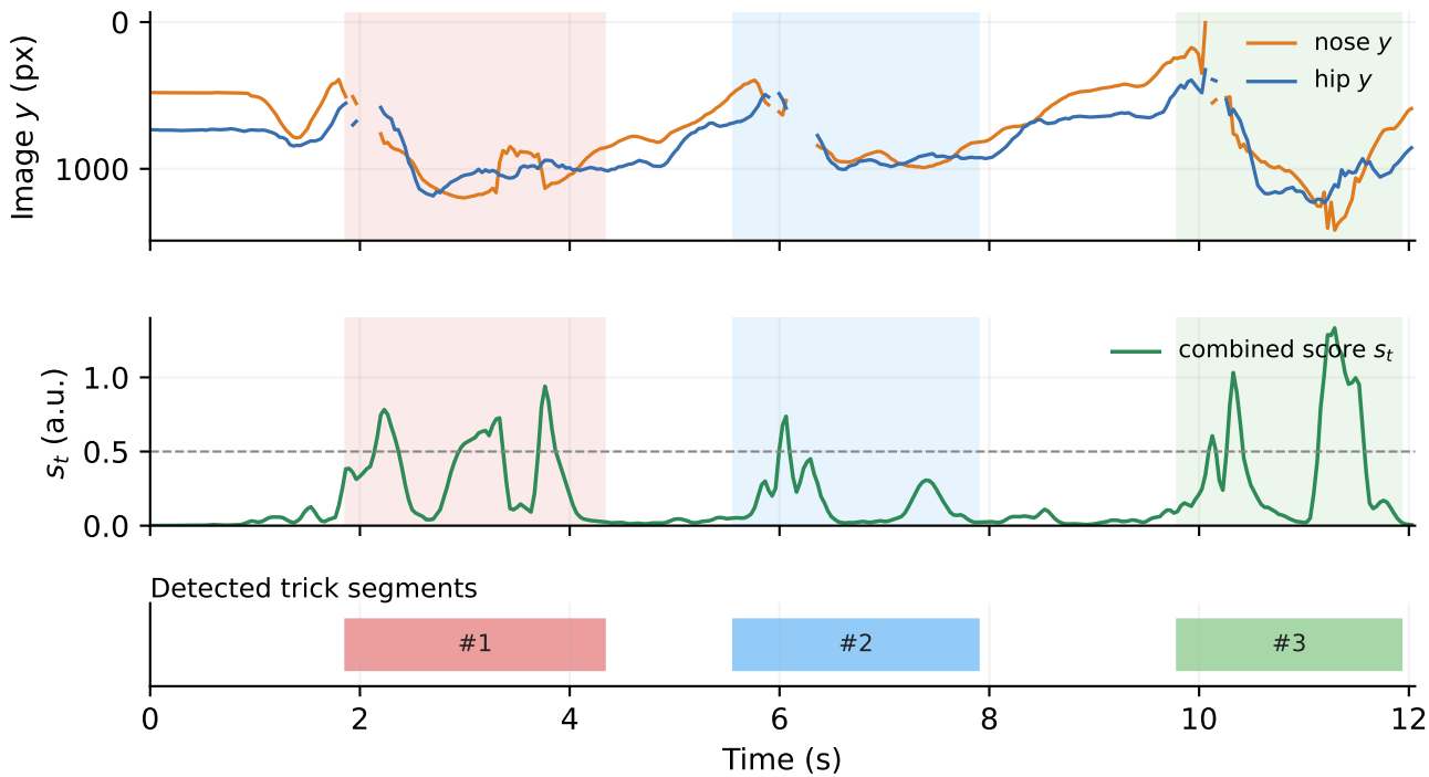
Inversion-based segmentation on \texttt{IMG\_5985.mov}
