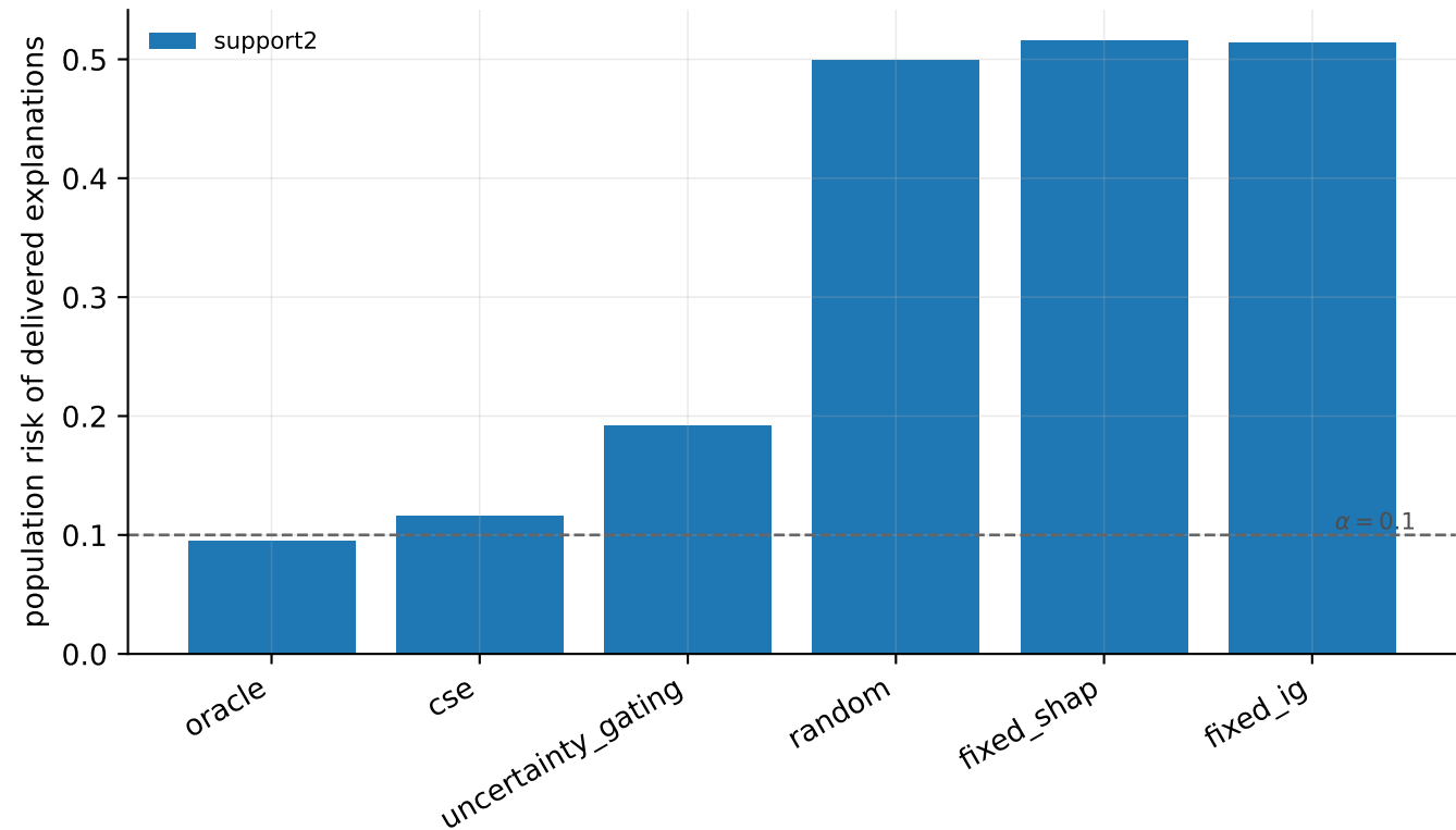
Policies at matched coverage (lower is better), \alpha = 0.1
