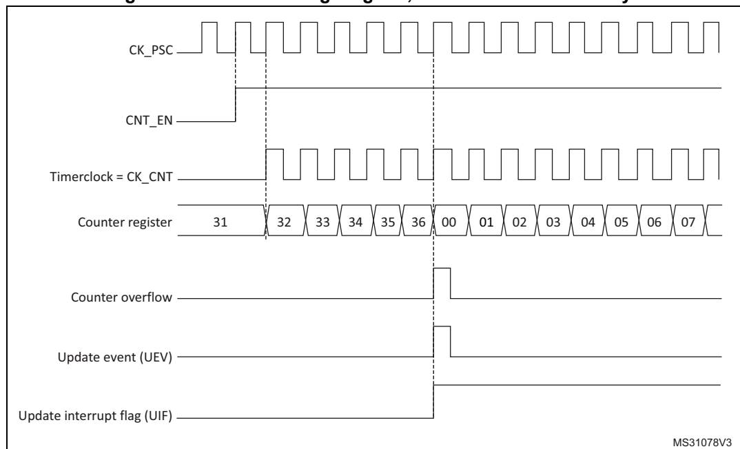
Figure 89. Counter timing diagram, internal clock divided by 1
