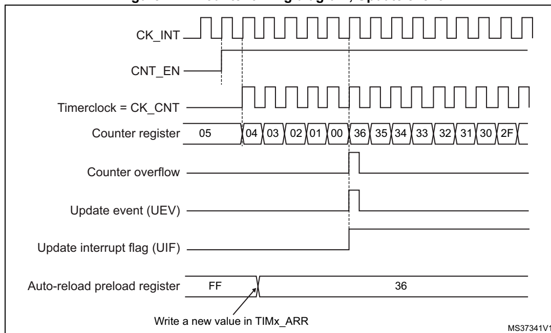
Figure 147. Counter timing diagram, Update event
