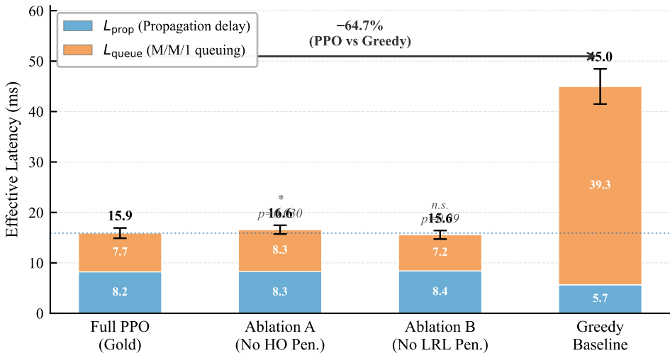
Fig. A: Effective Latency Comparison — All Routing Policies (N=20 episodes, M/M/1 model)
