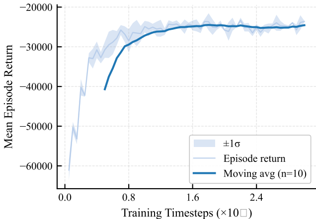
Fig. 1: PPO Training — Learning Curve
