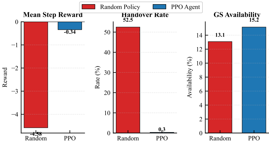
Fig. 4: PPO Agent vs. Random Policy — Key Metrics
