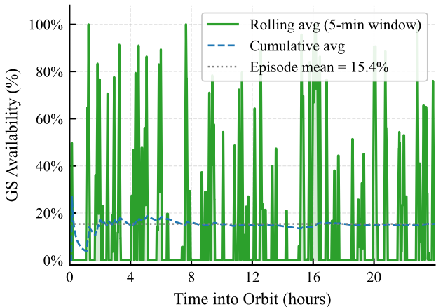
Fig. 5: Ground Station Availability — 24-Hour Orbit
