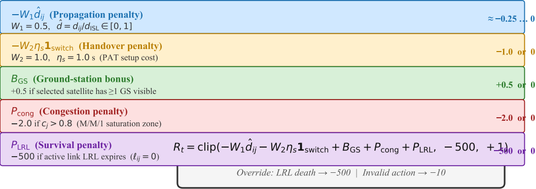
Fig. 7: Reward Function Decomposition — 5-Component Architecture
