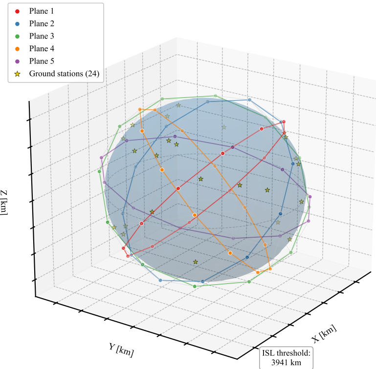
Fig. B: Walker Delta 60/5/1 Constellation 550 km · 53° · J2-perturbed · ISL links at epoch
