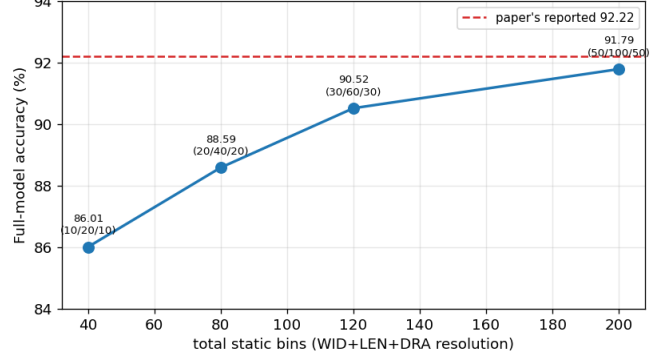
Fig 3.1 One undisclosed knob moves the headline 86 \rightarrow 92 Finer static bins alone recover the paper's number
