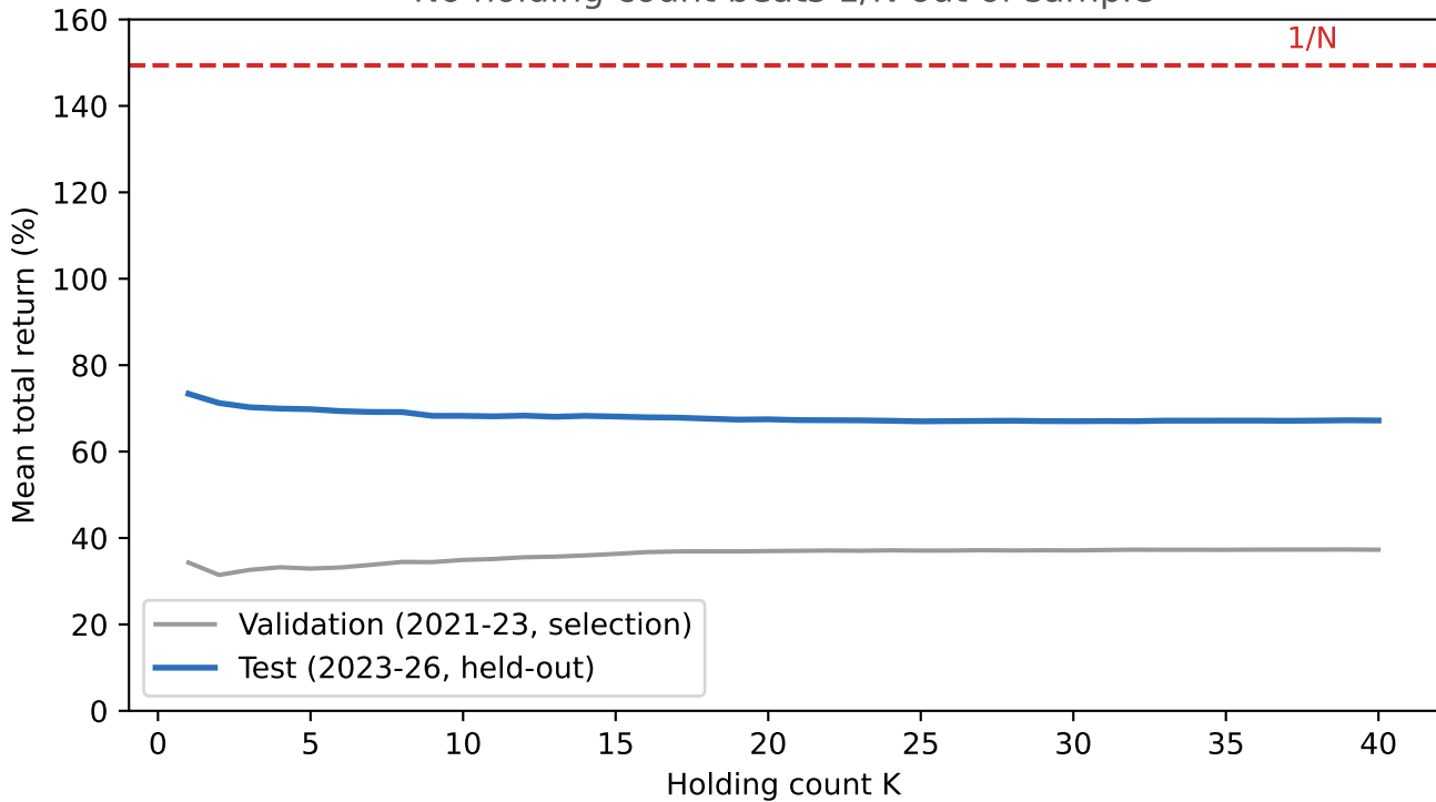
No holding count beats 1/N out of sample
