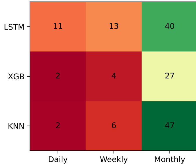
Beats 1/N on Calmar (%)
