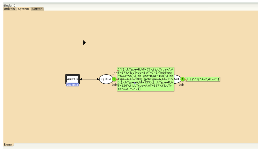
Рис. 3.9: System
