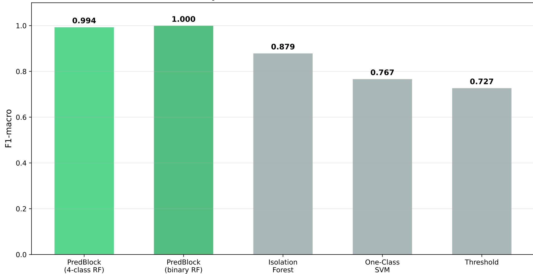
Anomaly Detection: PredBlock vs Baselines
