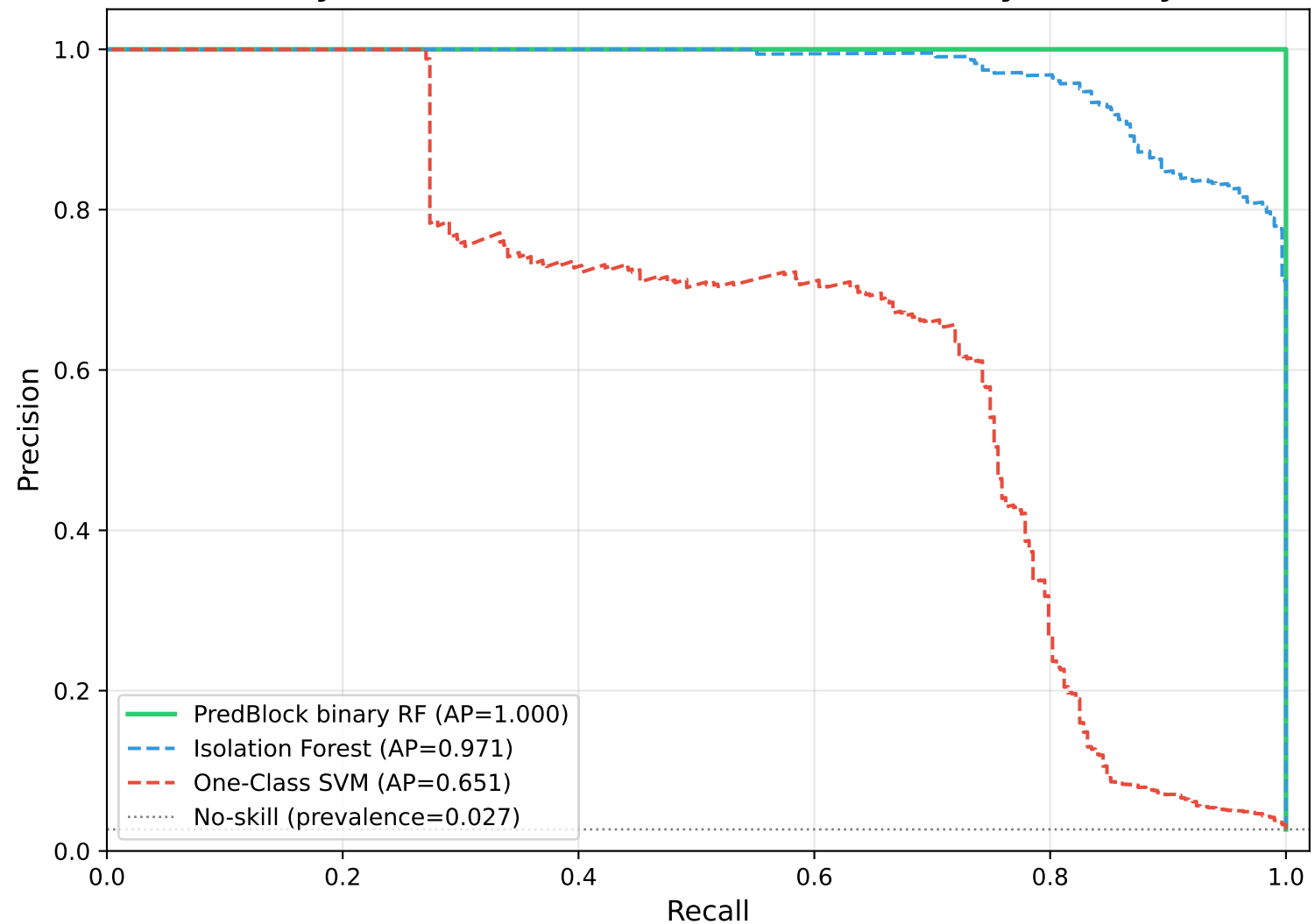
Binary Precision-Recall Curves (Normal vs Any Anomaly)
