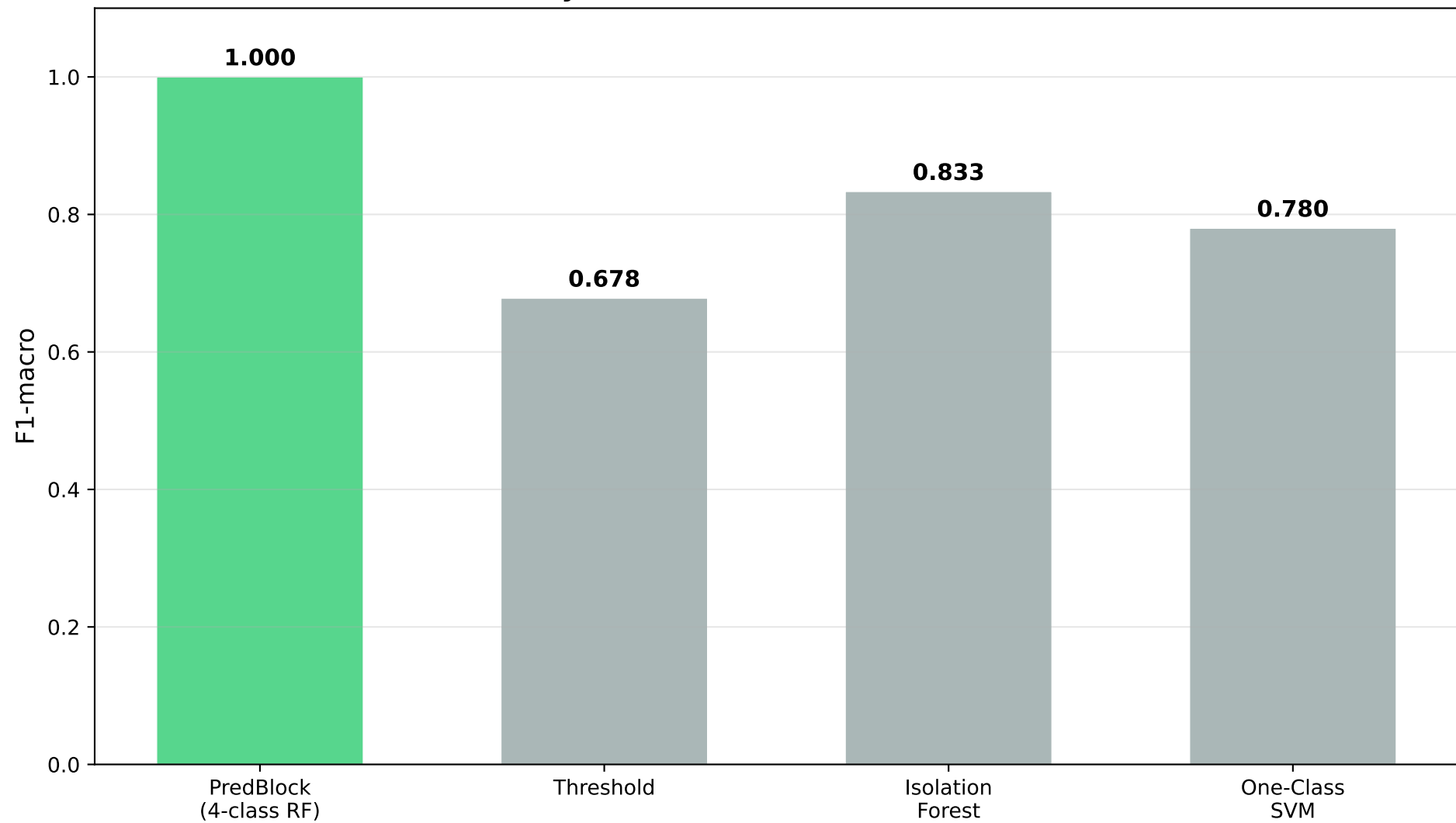
Anomaly Detection: PredBlock vs Baselines
