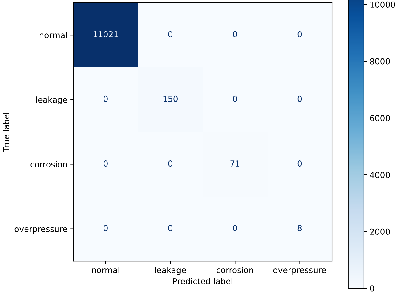
Confusion Matrix — PredBlock Multiclass Anomaly Detector
