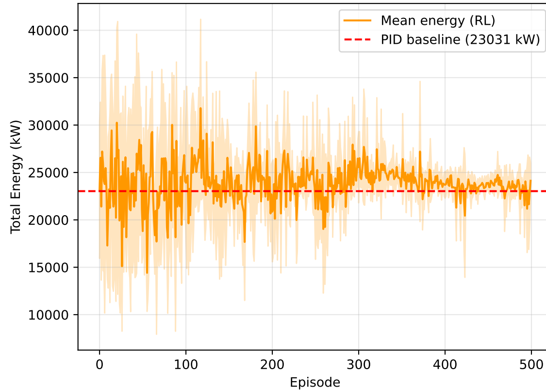
Energy Consumption per Episode
