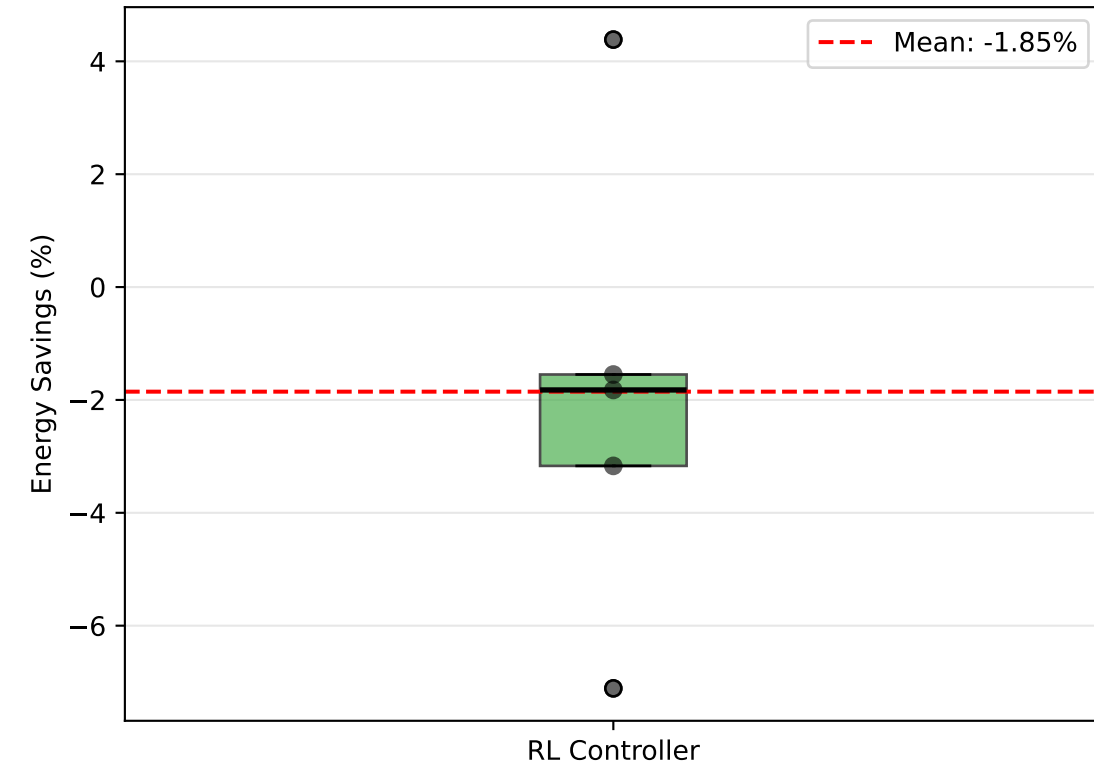
RL vs PID — Energy Reduction
